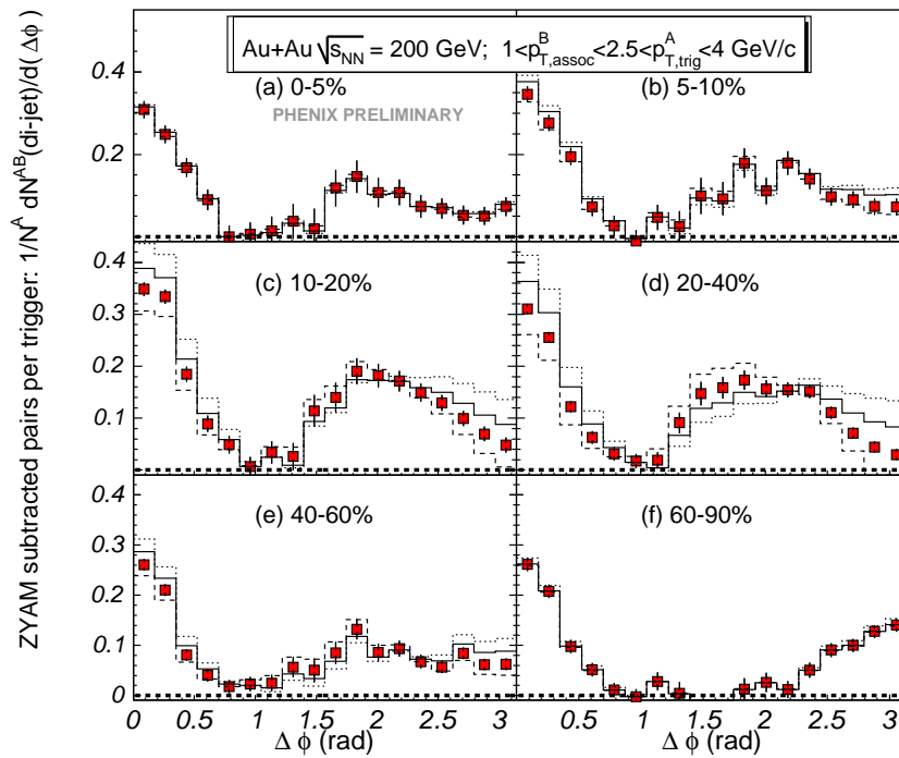
Fig. 4. ZYAM-subtracted jet-pair distributions 1/N_{trig}dN/d(\Delta\phi) . The dashed(solid) histograms indicate the distributions resulting from increasing(decreasing) v_2 = v_2^A \times v_2^B by one interval of the systematic error.
